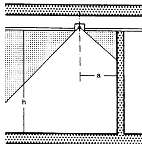
② Downlight, distance from wall: a = 1/3h
